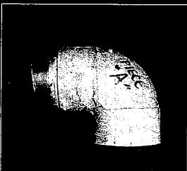
A fatality resulted when soldering on both ends of this elbow melted.
